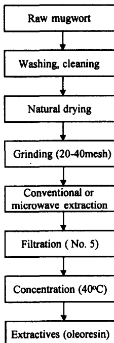
Fig. 1. Flow sheet for extractives production from mugwort.
